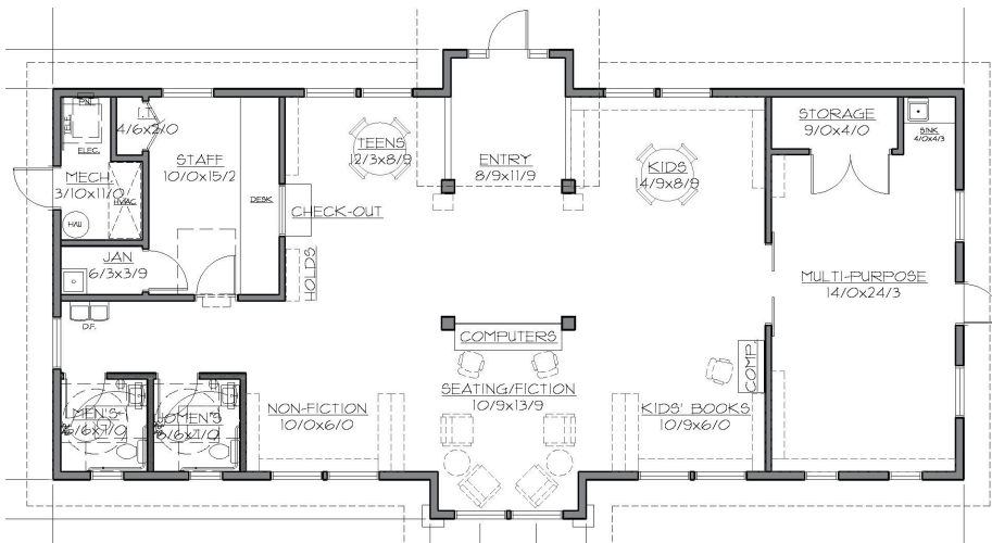
Preliminary Floor Plan for Proposed Yale Valley Community Library
